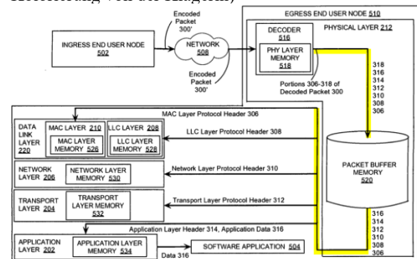
FIG. 5 (PRIOR ART)
